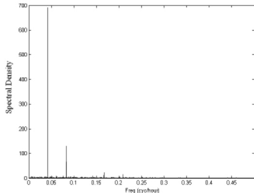
Figure 5 – Spectral periodgram for detached dwelling for metered profile over a six month period
