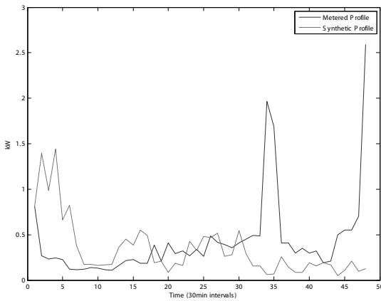
Figure 7 – Detached dwelling daily profile for 01 st July 2009
