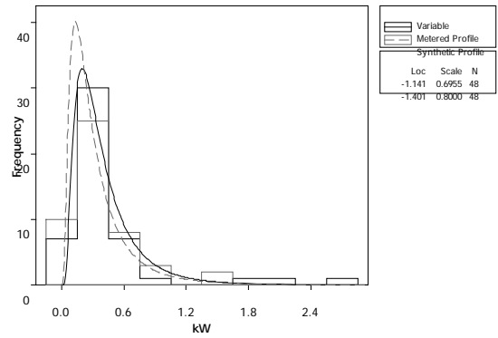
Figure 8 – Detached dwelling daily histogram for 01 st July 2009
