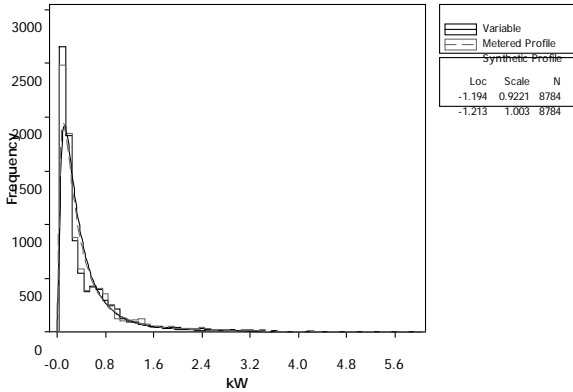
Figure 2 – Detached dwelling histogram for metered and synthetic profiles over six months
