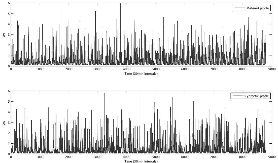
Figure 1 – Detached Dwelling Six Month Profile
